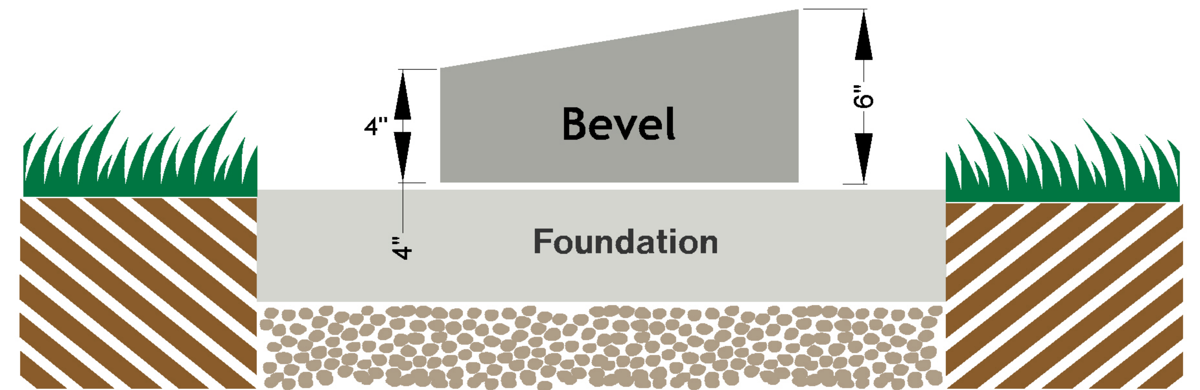
Bevel Side View - No Base 4" in Front & 6" in Back
