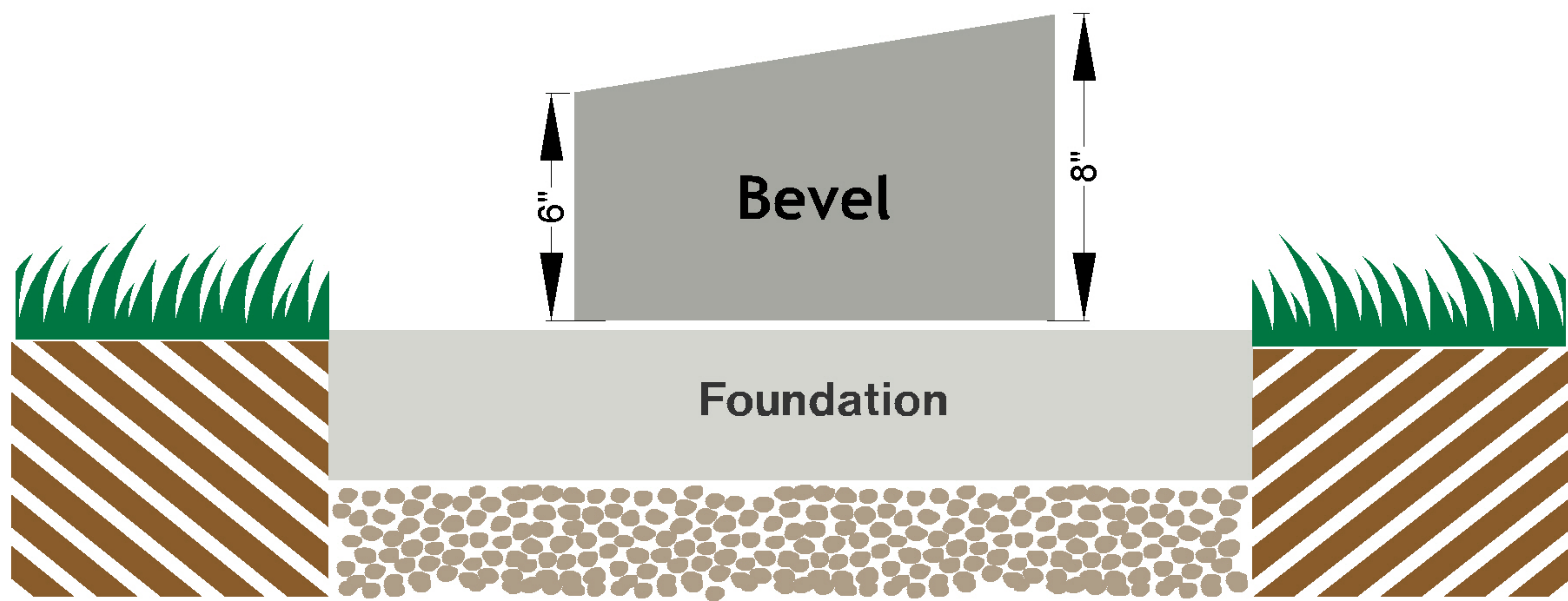
Bevel Side View - No Base 6" in Front & 8" in Back
